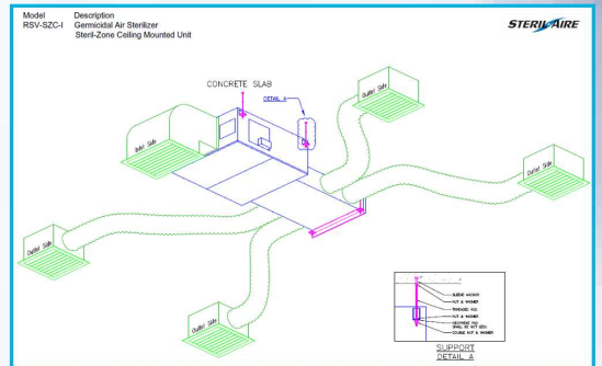
Classrooms (Germicidal Air Sterilizer installation Detail) 教室(殺菌空氣消毒機安裝詳情)
