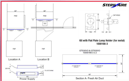
Fresh Air Duct (UVC Emitter Installation Layout) 鮮風喉(UVC發射器安裝設置)
