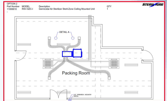
Packing Room (Germicidal Air Sterilizer installation layout) 包裝室(殺菌空氣消毒機安裝設置)
